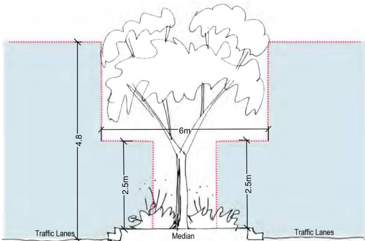
Figure SC6.7-3: Clearance zone under powerlines
