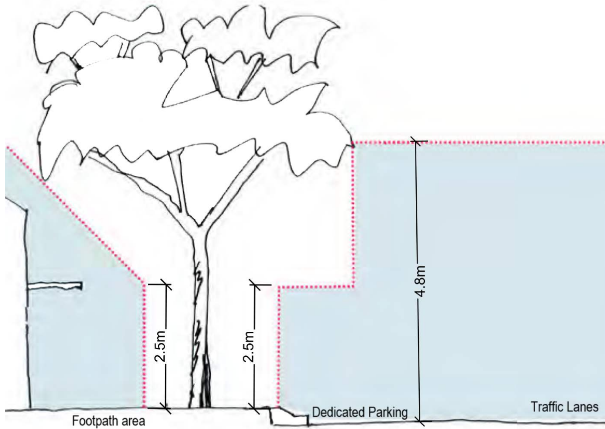
Figure SC6.7-1: Clearance zone along street verge
