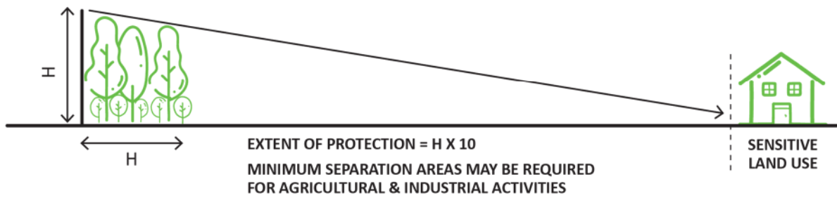
Figure SC6.7-5: Buffer density of screen landscaping
